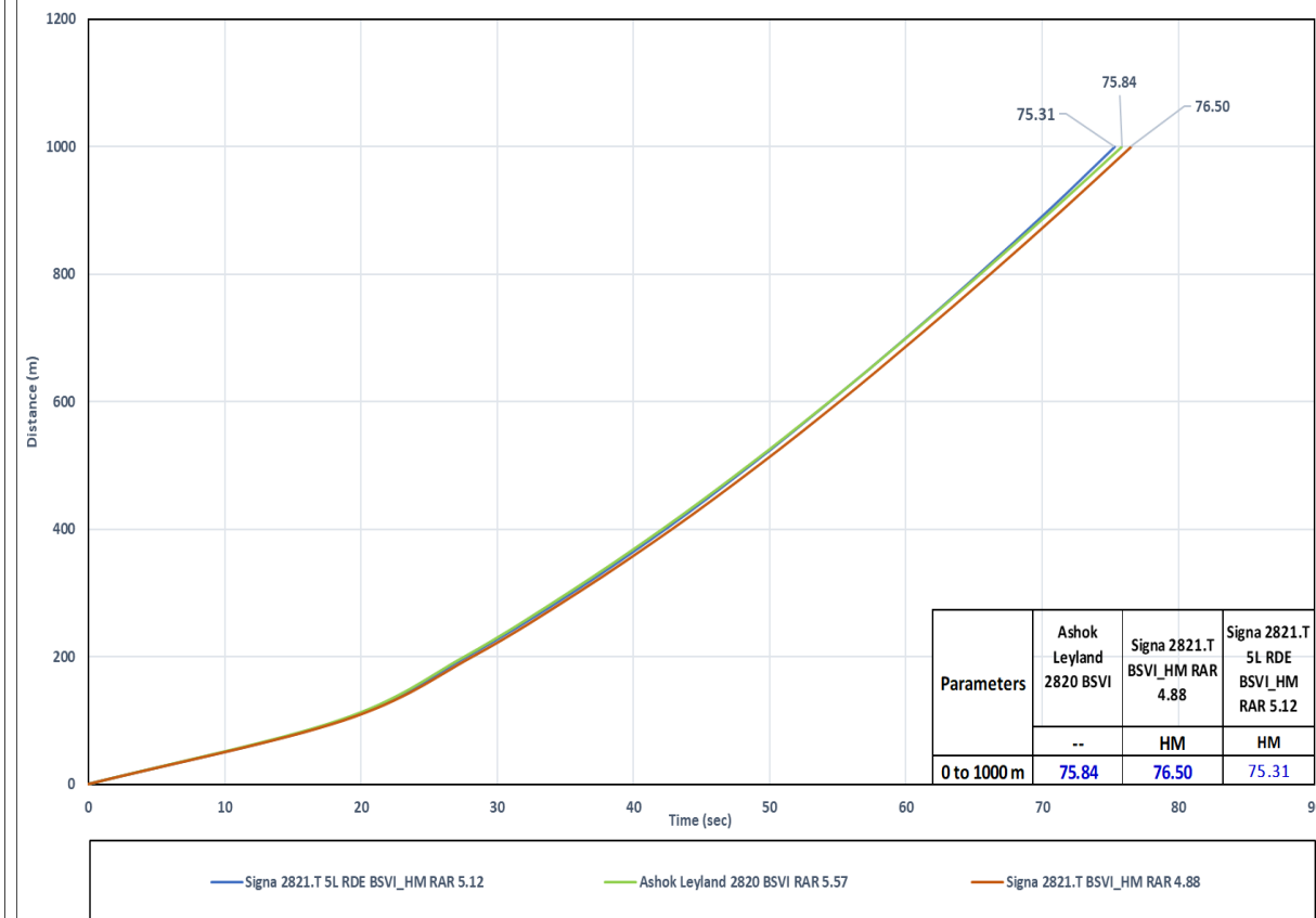
Acceleration 0 to 1000m
