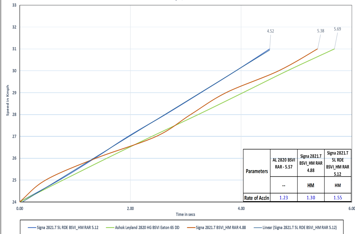
Drivability @ 4 th Gear
