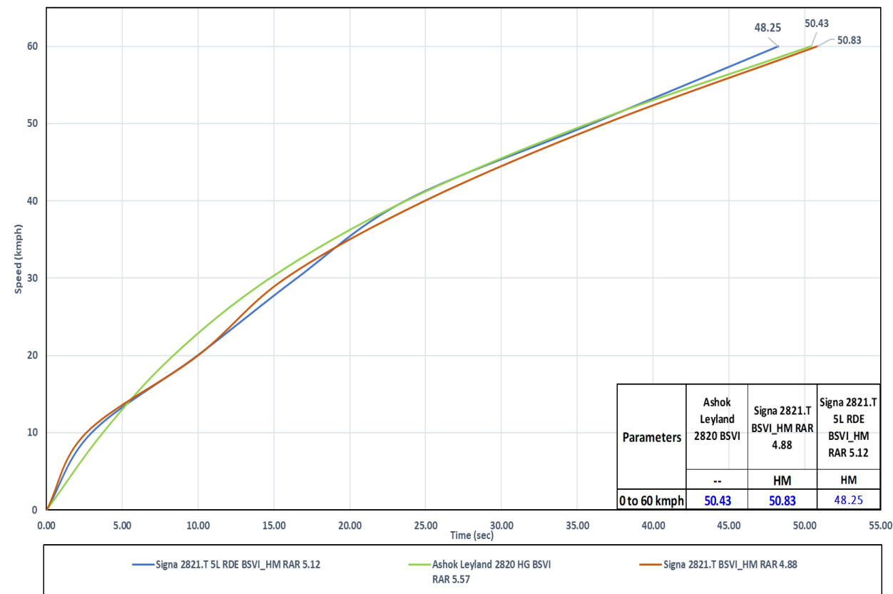
Acceleration 0 to 60kmph
