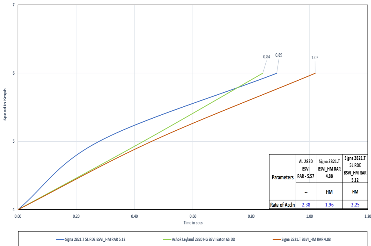
Drivability @ 1st Gear
